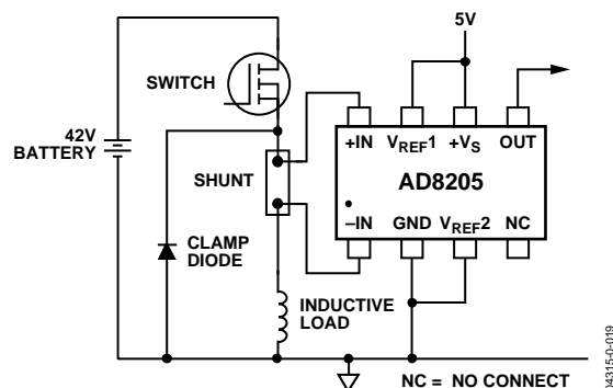
Figure 20. High-Side Switch
