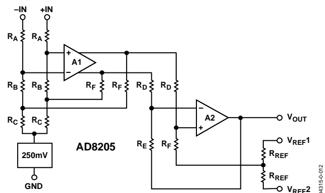
Figure 13. Simplified Schematic
